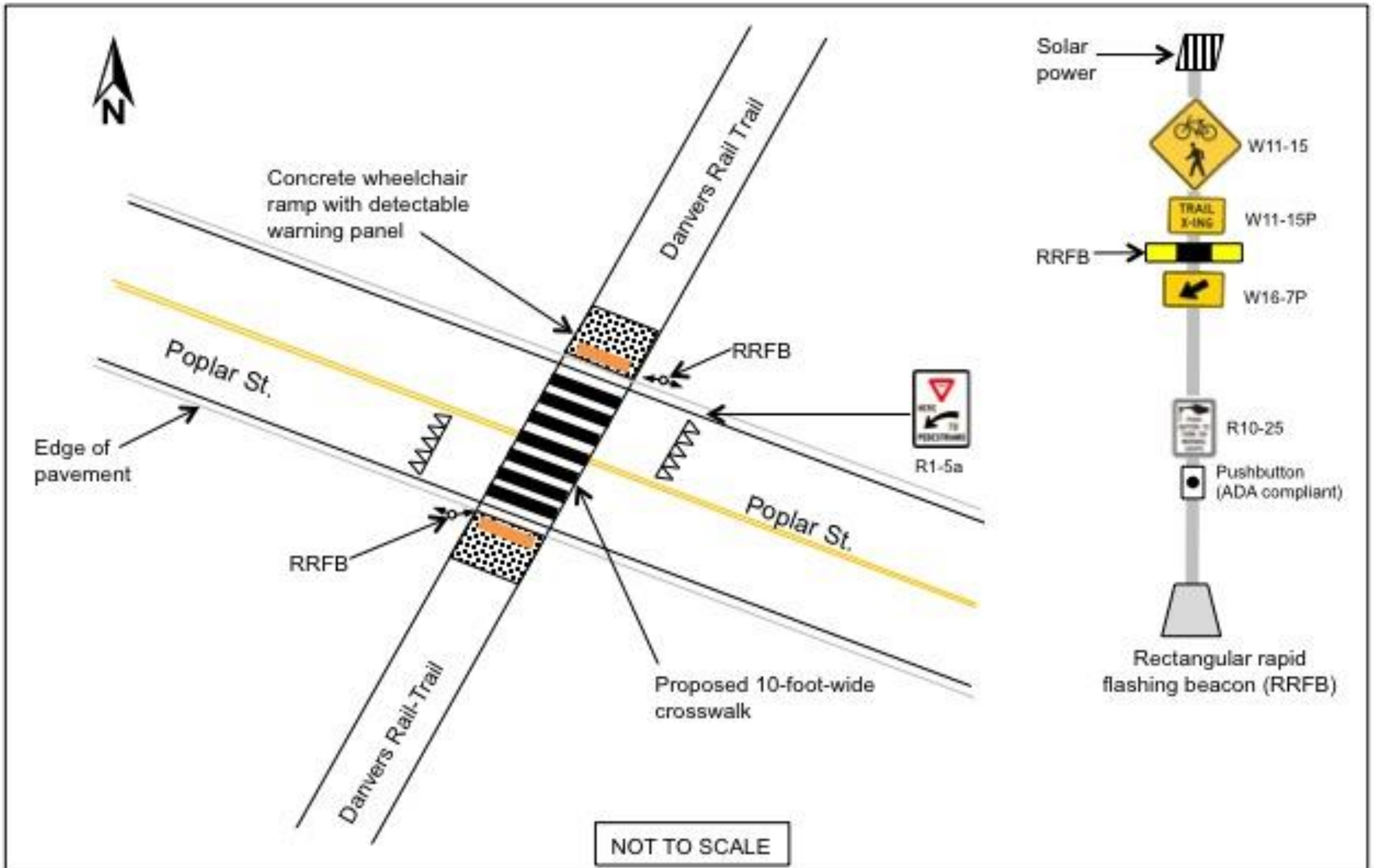
FIGURE 6 Rectangular Rapid Flashing Beacon and Crosswalk Assembly
